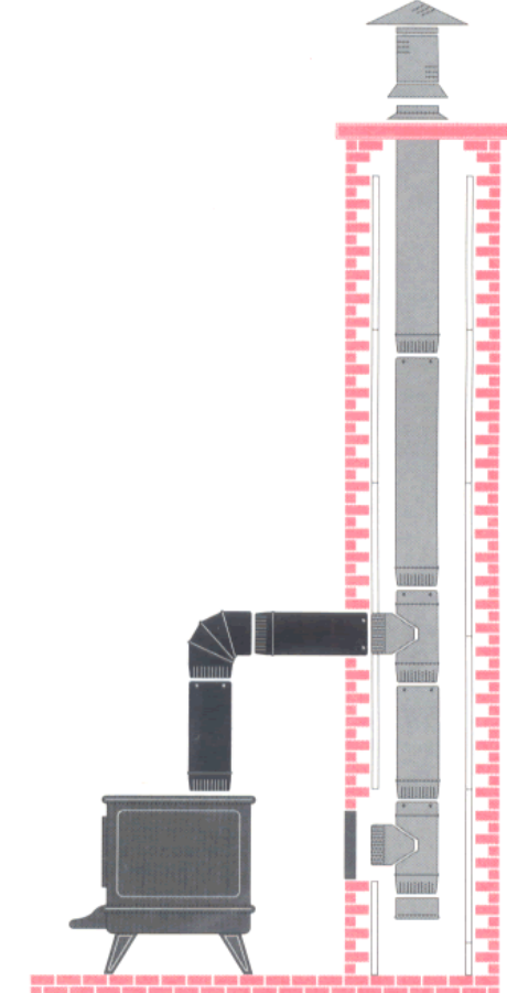
FREESTANDING SOLID FUEL STOVE INSTALLATION
