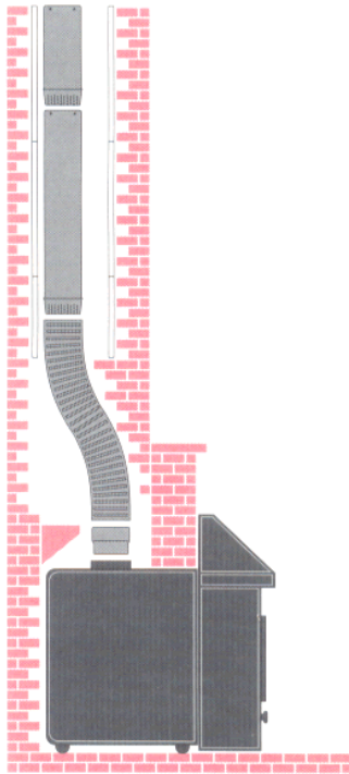
FIREPLACE INSERT INSTALLATION
