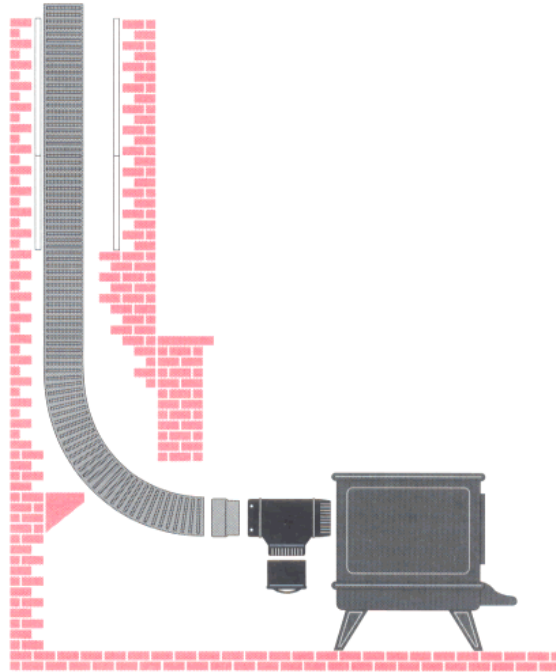
HEARTH STOVE INSTALLATION
