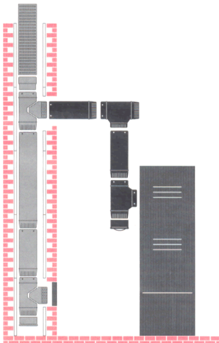
SOLID FUEL, OIL OR GAS FURNACE INSTALLATION
